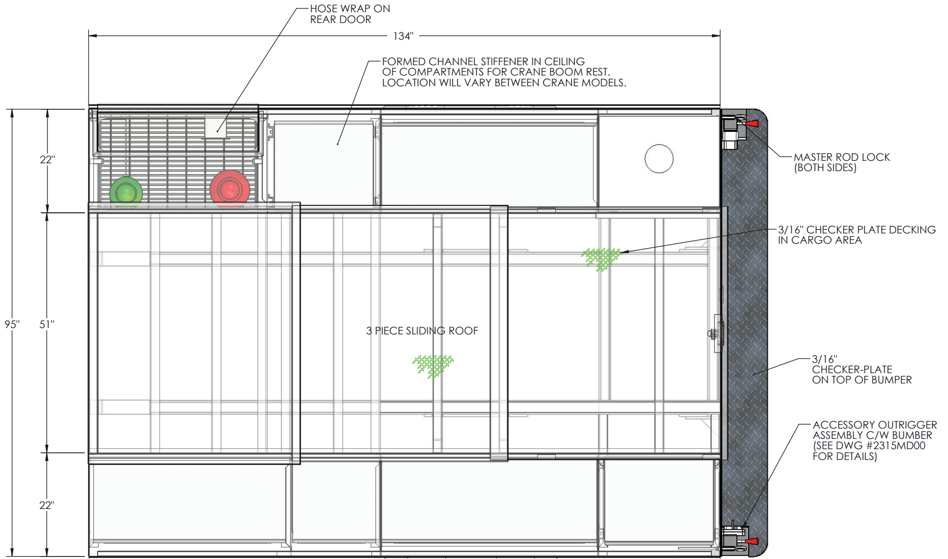
PLAN VIEW
